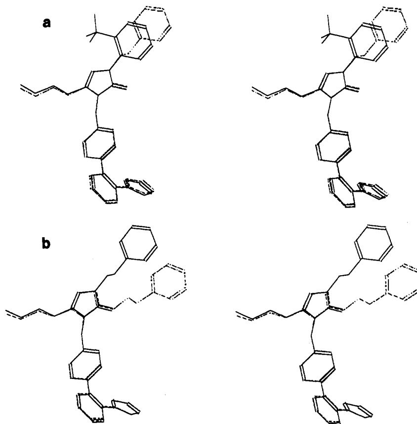
Figure 1. Stereoviews of computer-generated, energy-minimized conformations of AII antagonists: (a) overlay of triazolones 25 (solid) and 81 (dotted); (b) overlay of triazolone 81 (solid) and triazole 107 (dotted).
